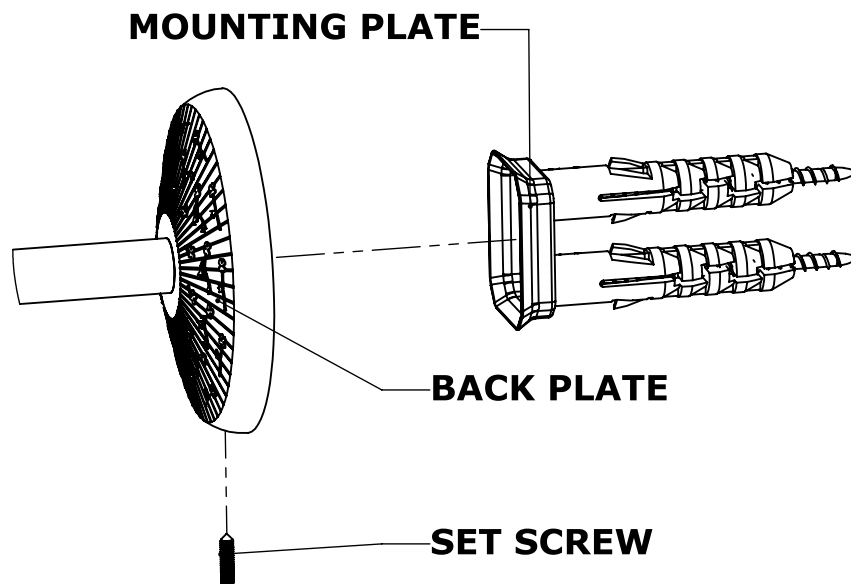
DETAIL N
